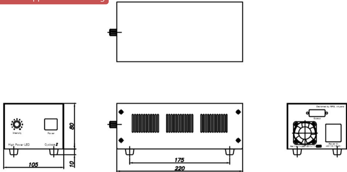
Controller appearance drawing
