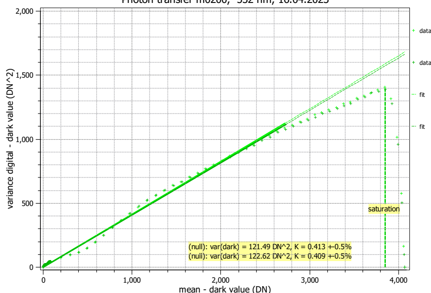
Photon transfer m0200, 532 nm, 16.04.2023
