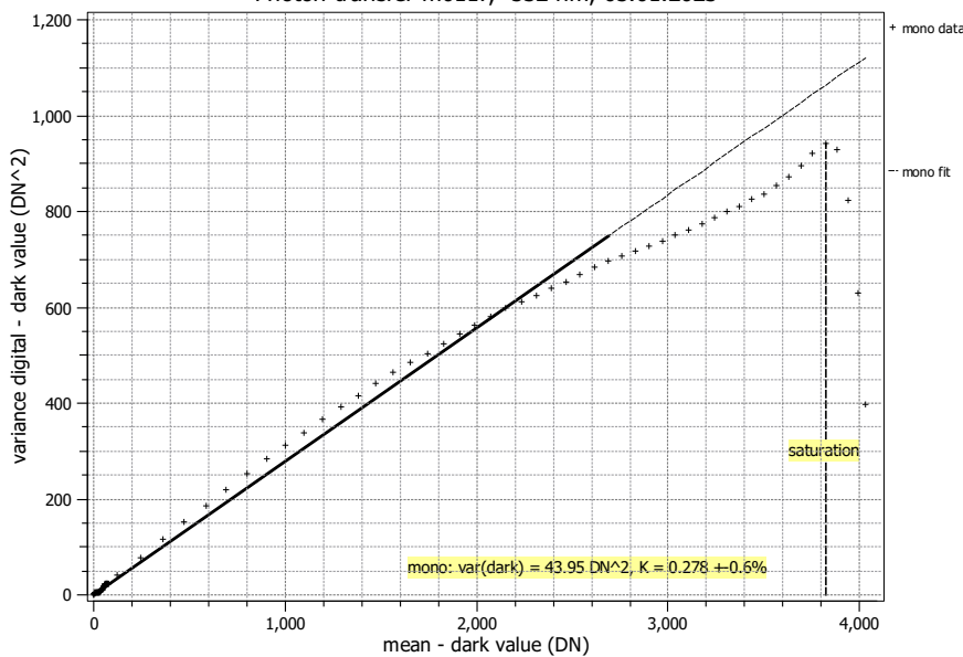
Photon transfer m0117, 532 nm, 05.01.2023
