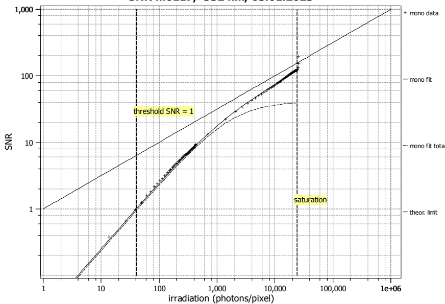
SNR m0117, 532 nm, 05.01.2023
